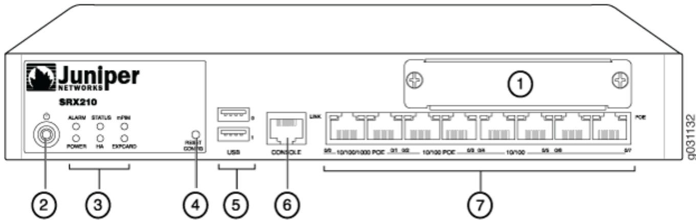
Figure 1 - Juniper Networks SRX210 Front Panel
