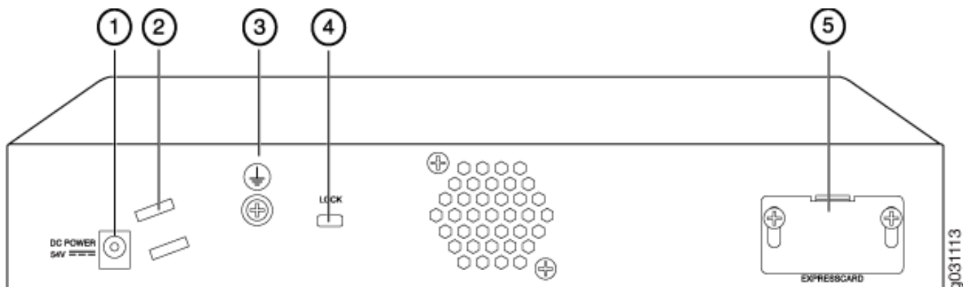
Figure 2 - Juniper Networks SRX210 Back Panel
