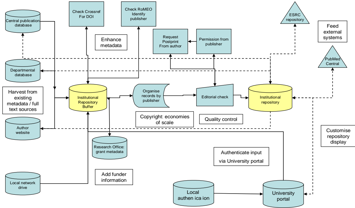
Figure 1: Repository ingest and outputs
